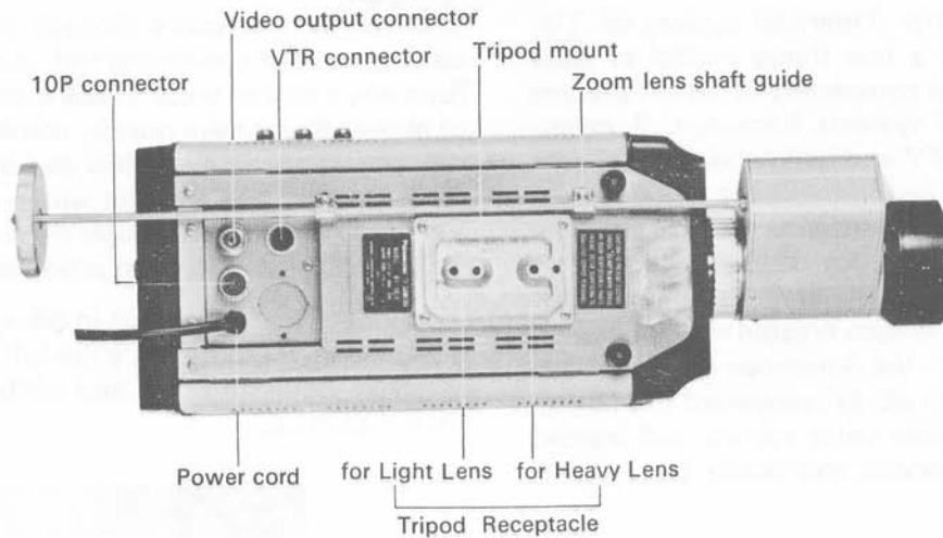
Camera Bottom View
