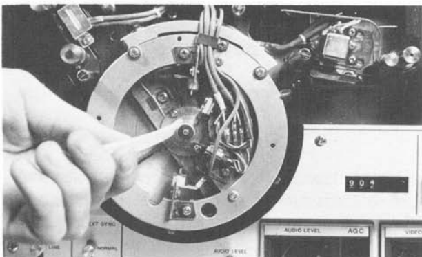
Cleaning The Slip Rings
