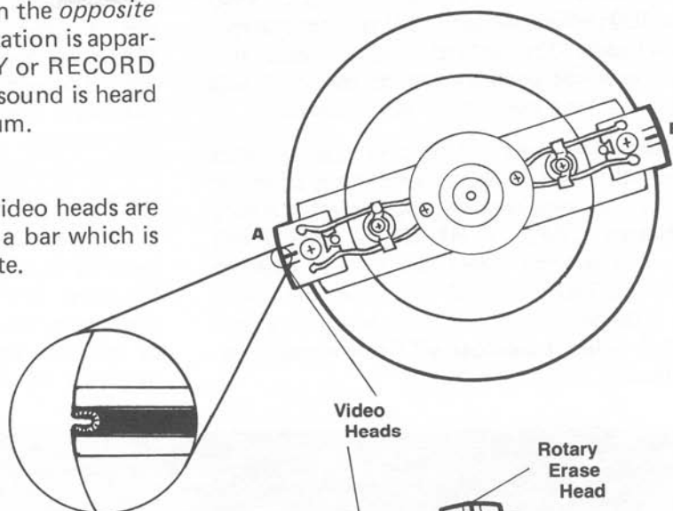
EIAJ Video Head Assembly
