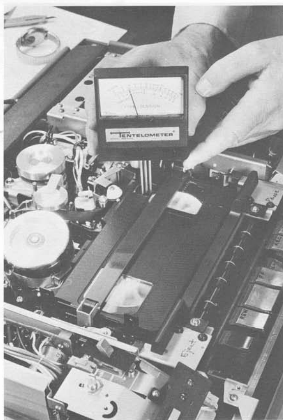
Tentel Tension Gauge
