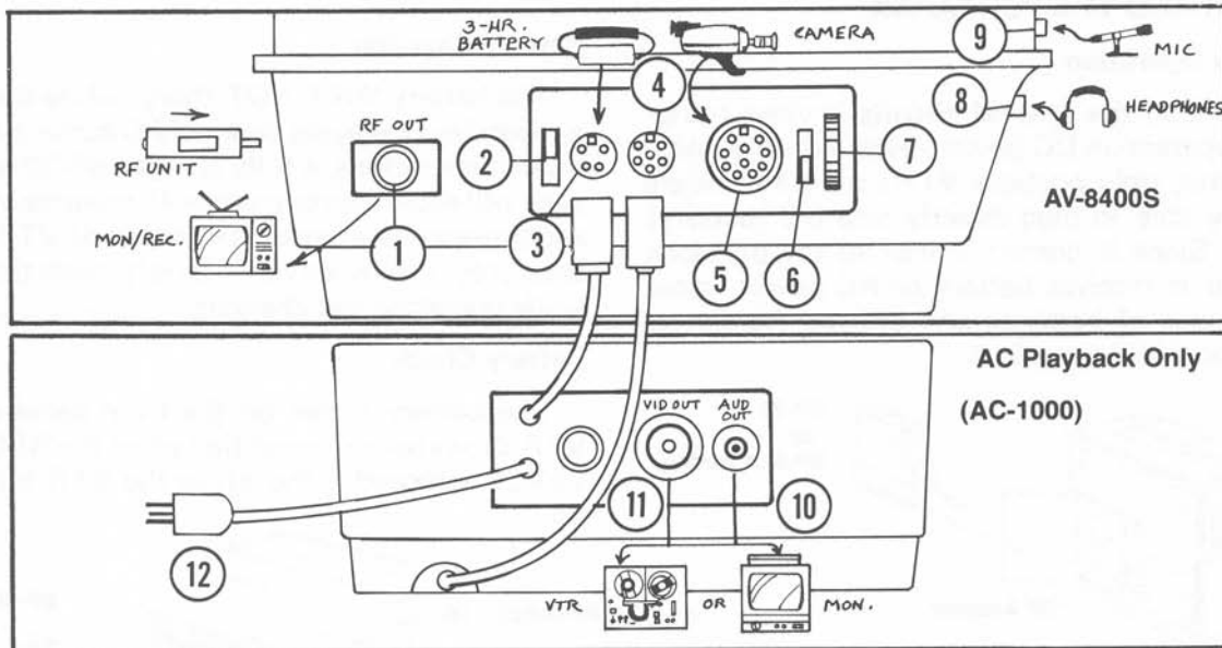
AV-8400S Side View—Input Output Panels
