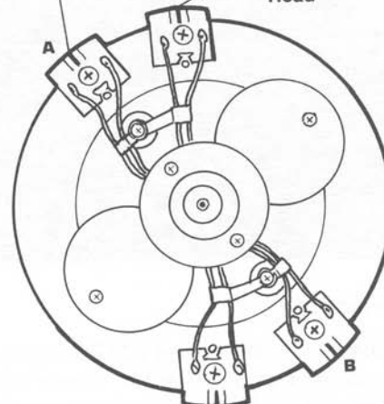
Sony AV-8650 With Rotary Erase Heads
