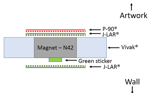
Fig. 3. Profile diagram of strip construction
