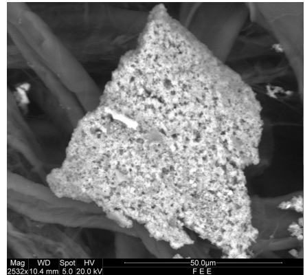
Fig. 7. Moderate corrosion of large iron deposits with very little corrosion on surrounding fibers: sample 10, localized treatment with 2% SDT and DTPA at 2532xM, working distance 10.4mm, sample 10 area 4. Image taken by Kayleigh Fuller, Conservation Program staff.
