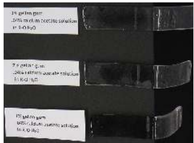
Fig. 4. Comparison of rigidity of gellan gum concentrations incorporating calcium acetate.
