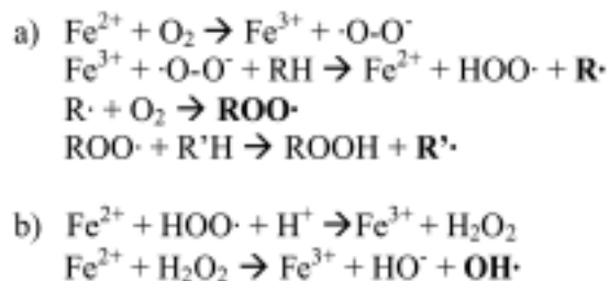
Fig. 5. The oxidative degradation of cellulose catalyzed by iron (II): a) the direct production of organic radicals and their subsequent oxidation, b) the Fenton reaction, or the production of hydrogen peroxide and its decomposition to a hydroxyl radical and a hydroxide ion
